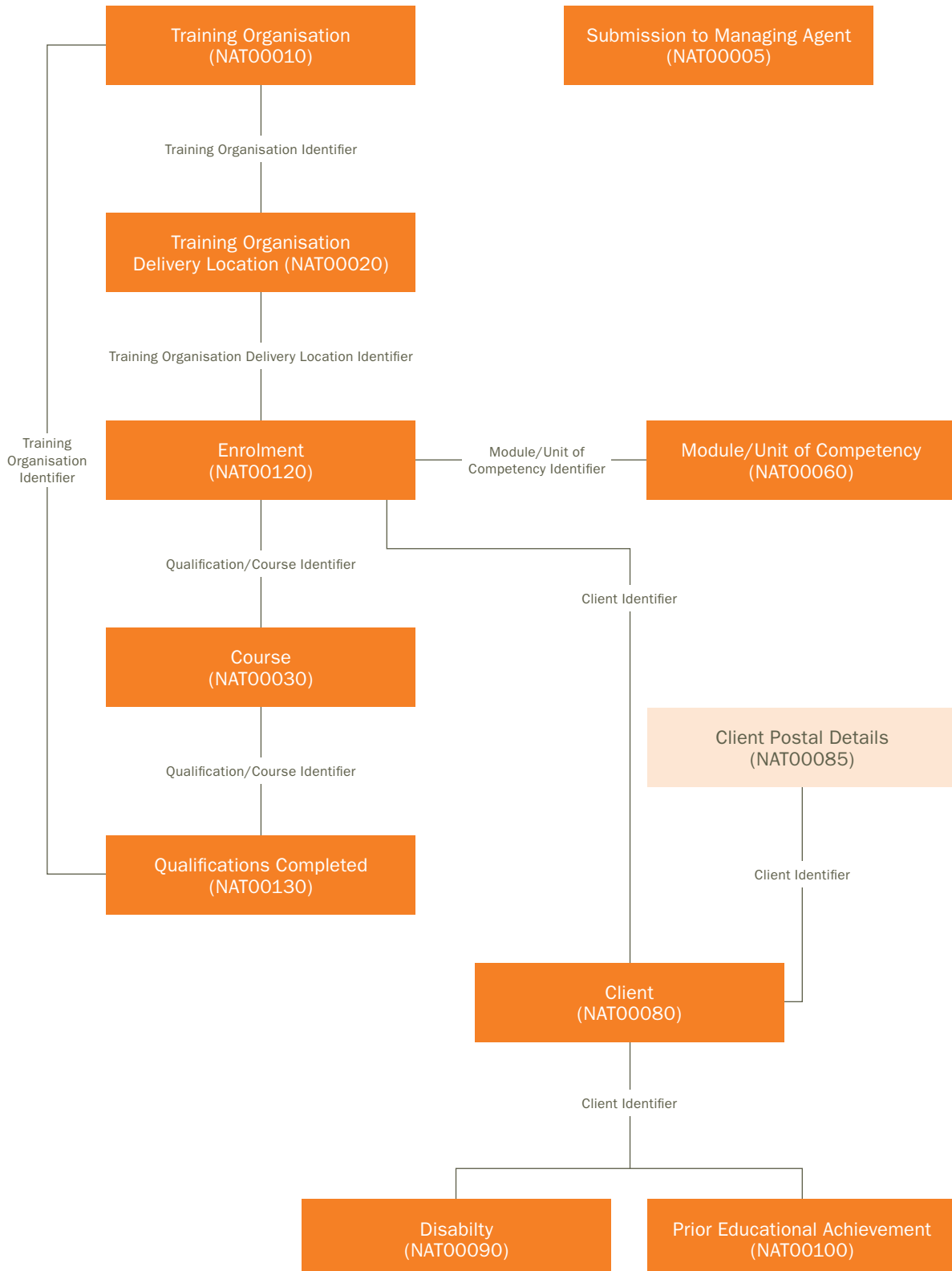
Figure 2: Entity Relationship Diagram (ERD) between the national VET provider collection tables
